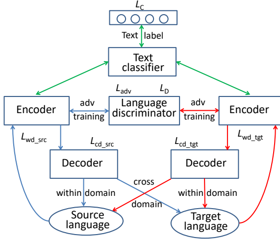
Figure 1: Multi-view encoder classifier (MVEC) architecture. Blue (red) lines indicate the message flow within source/target language (across languages) respectively. Green lines indicate the message flow from the encoder for the text classifier. The encoder-decoder shares the same parameters for two languages.
