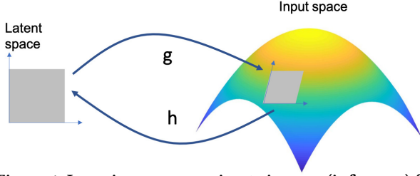
Figure 1: Learning an approximate inverse (inference) function of the generator.
