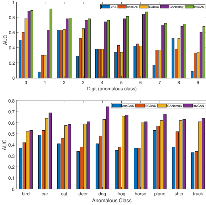
Figure 4: Anomaly detection with different models on the MNIST and CIFAR10 data sets.
