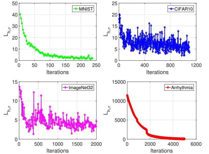
Figure 5: L_{h,\sigma} at different iterations for different data sets.
