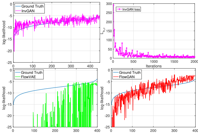
Figure 2: The upper left plot shows the InvGAN log-likelihoods of the simulated testing set; Upper right presents the objective loss values over iterations; The lower two plots give the log-likelihood values of the simulated data set using FlowVAE and FlowGAN. For plots with log-likelihood values, Y axe is the log-likelihood value, and X axe is sample index based on the increasing order of the ground truth log-likelihood value.
