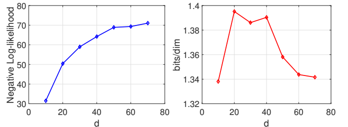
Figure 3: The left plot shows the average negative log-likelihood values of a MNIST testing image set using InvGAN at different latent space dimension ( d ). The right plot presents the corresponding bits/dim for the testing set under the revised metric at different d values.
